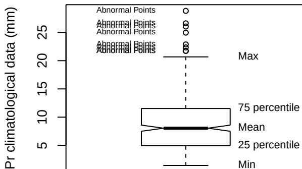
Box plot (STMC)
