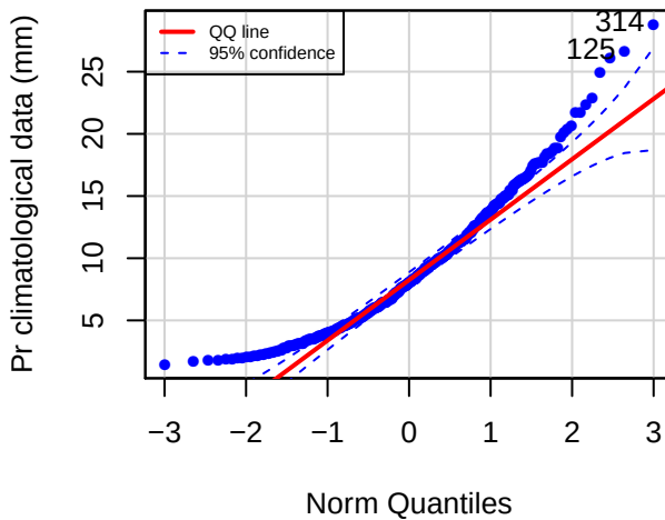
QQ plot (STMC)
