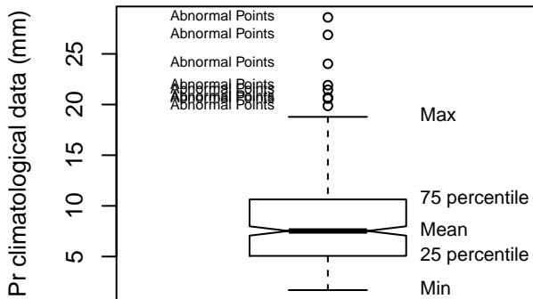
Box plot (STMM)
