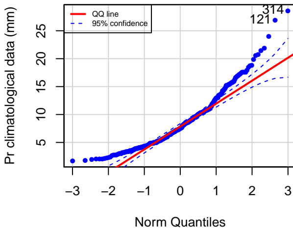
QQ plot (STMM)
