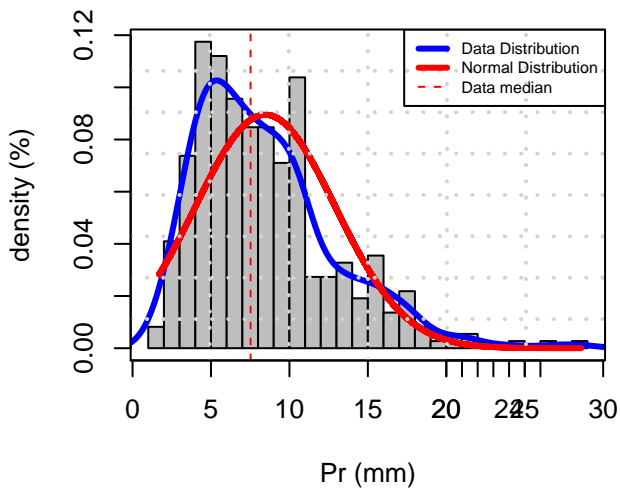
Histogram Distribution (STMM)
