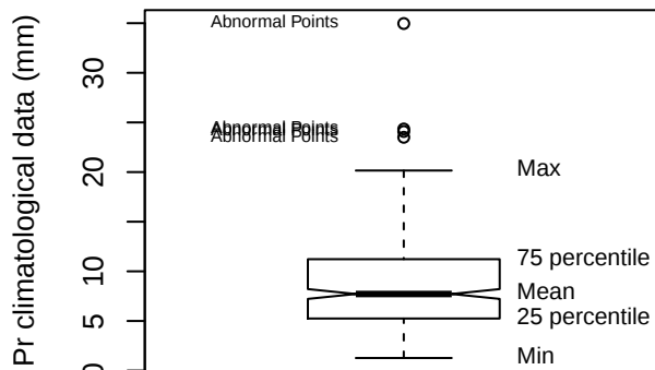
Box plot (STMP)
