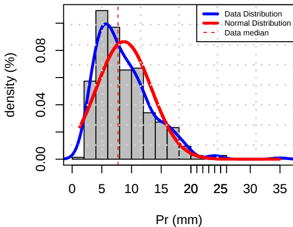
Histogram Distribution (STMP)
