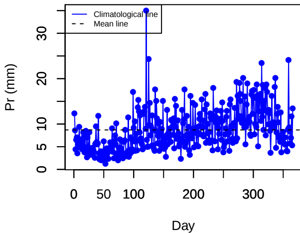
Climatology (STMP)
