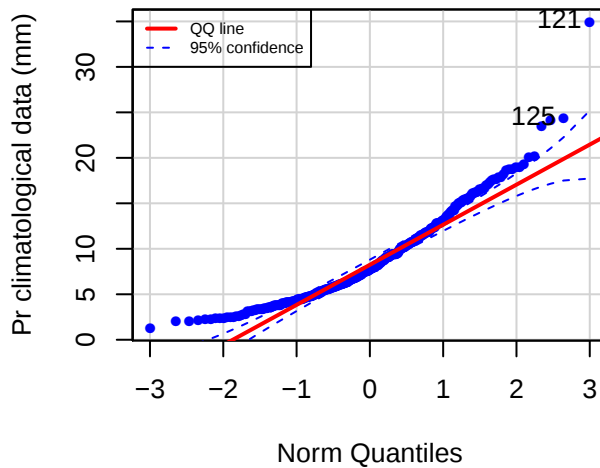
QQ plot (STMP)
