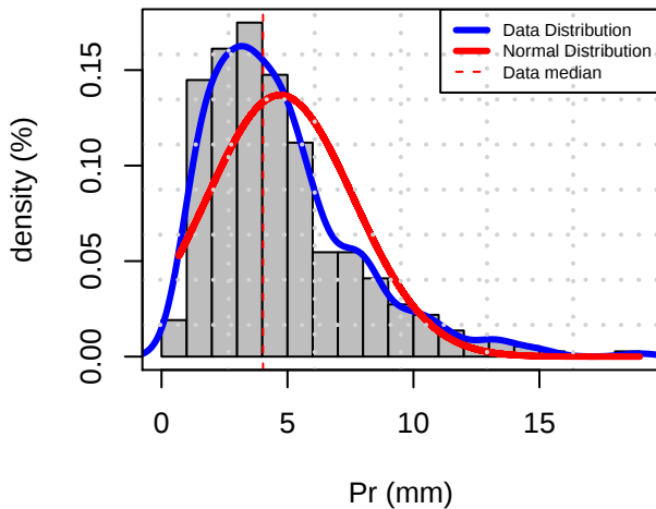
Histogram Distribution (TILG)
