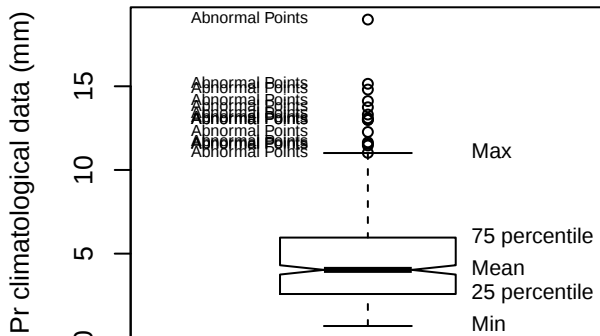
Box plot (TILG)
