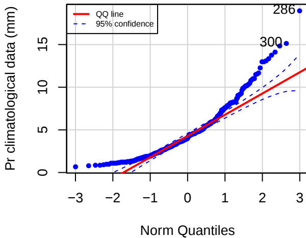
QQ plot (TILG)
