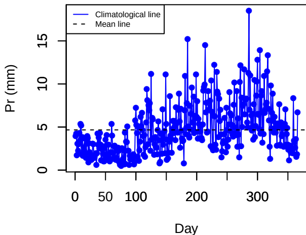
Climatology (TILP)
