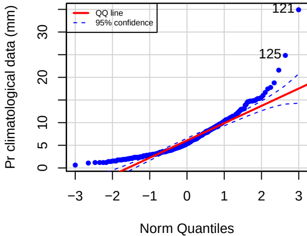
QQ plot (TRTR)
