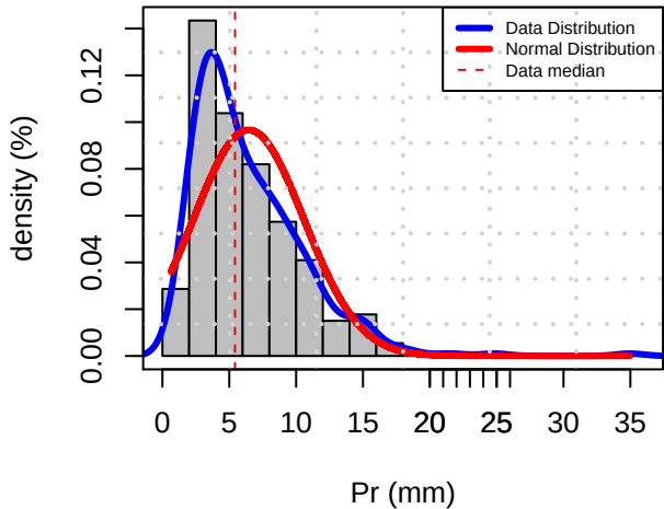
Histogram Distribution (TRTR)
