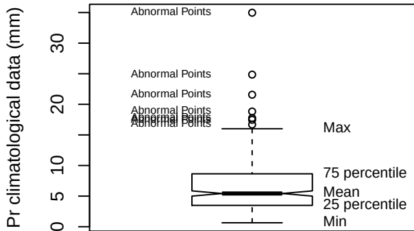
Box plot (TRTR)
