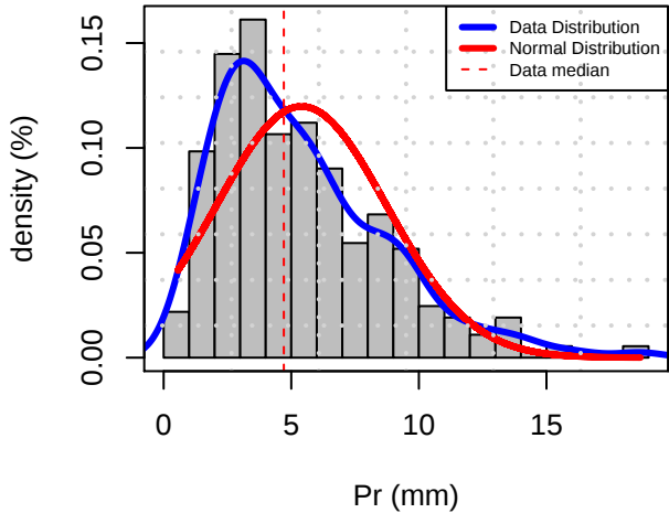
Histogram Distribution (TRTS)
