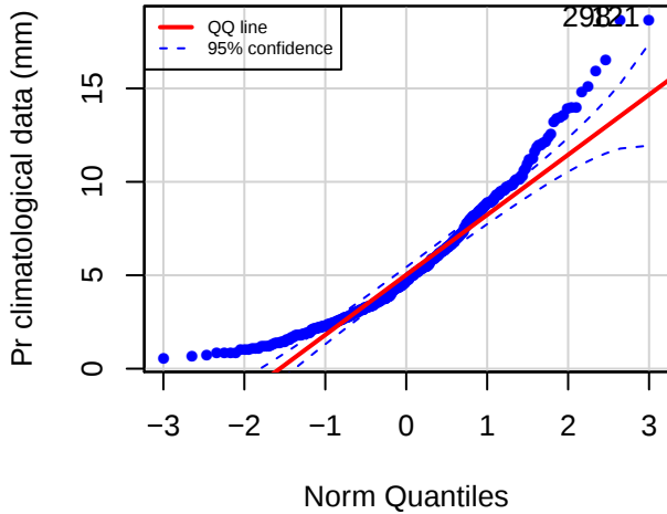
QQ plot (TRTS)
