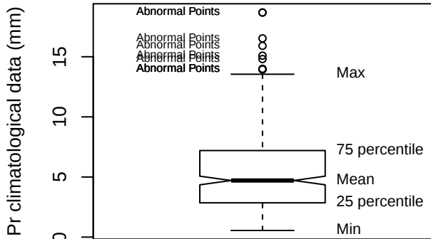
Box plot (TRTS)
