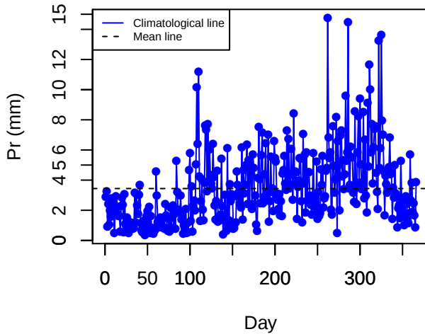
Climatology (VCLC)
