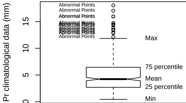
Box plot (VCLR)
