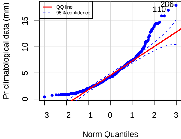
QQ plot (VCLR)
