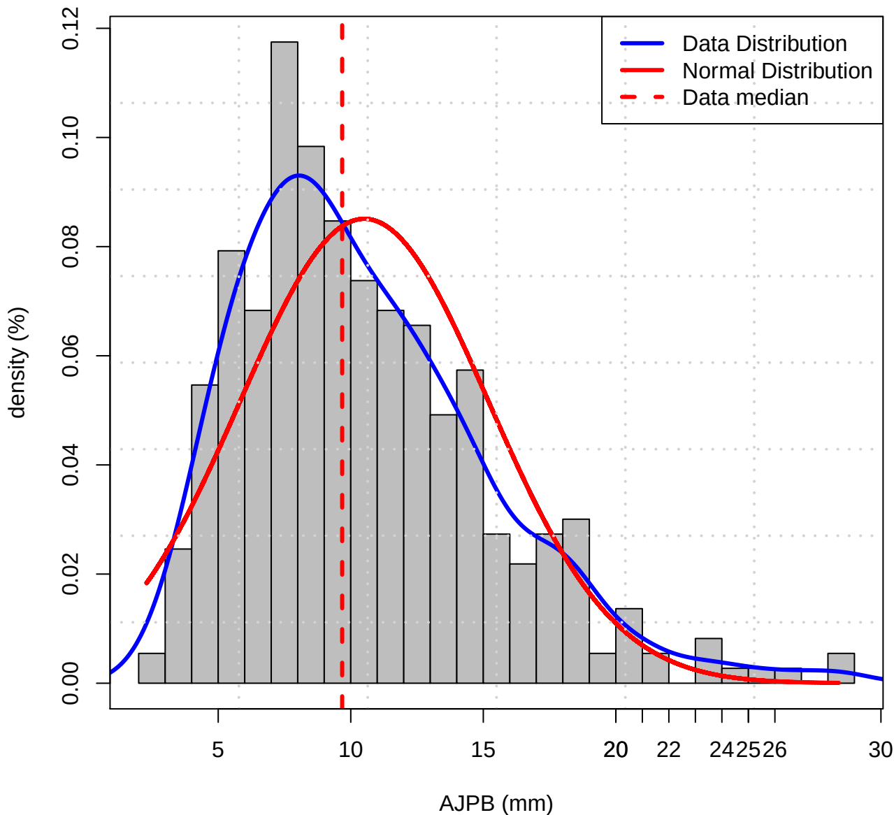
Histogram of Data distribution (PR of AJPB)
