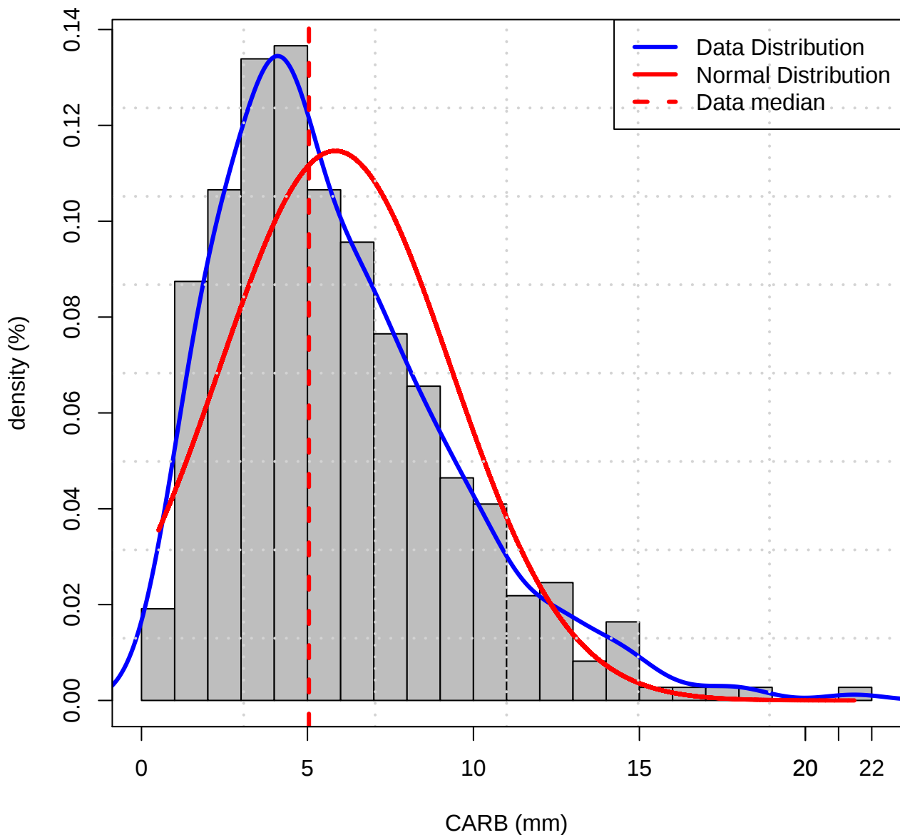
Histogram of Data distribution (PR of CARB)
