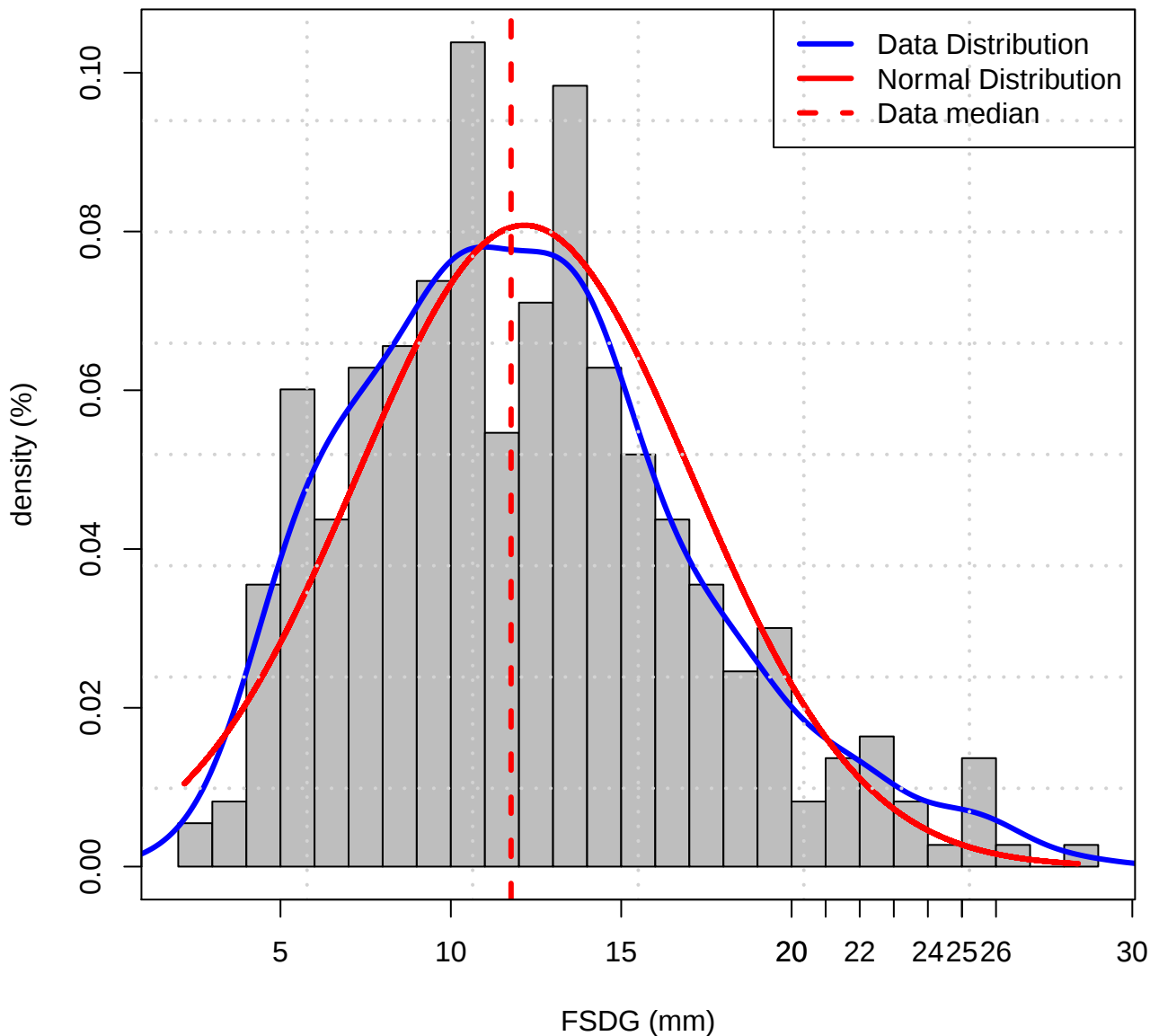
Histogram of Data distribution (PR of FSDG)
