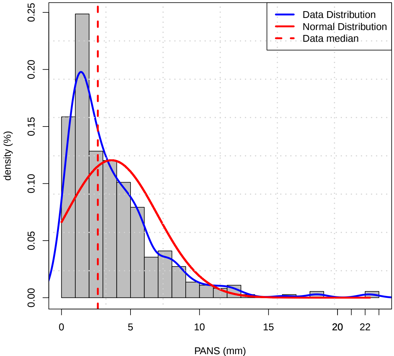
Histogram of Data distribution (PR of PANS)
