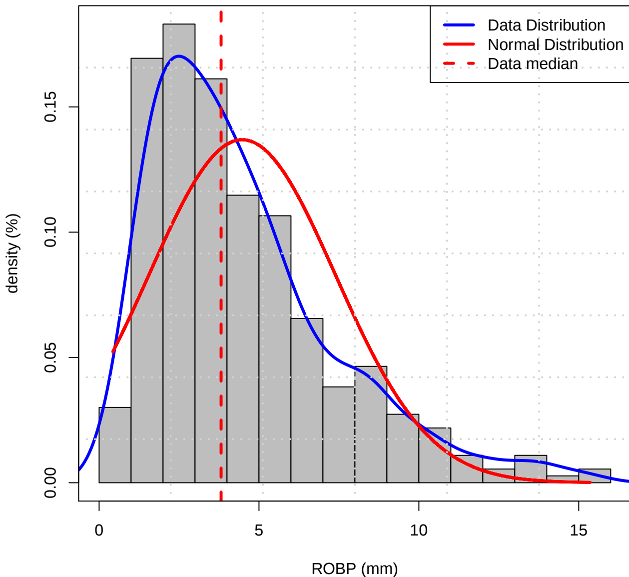
Histogram of Data distribution (PR of ROBP)
