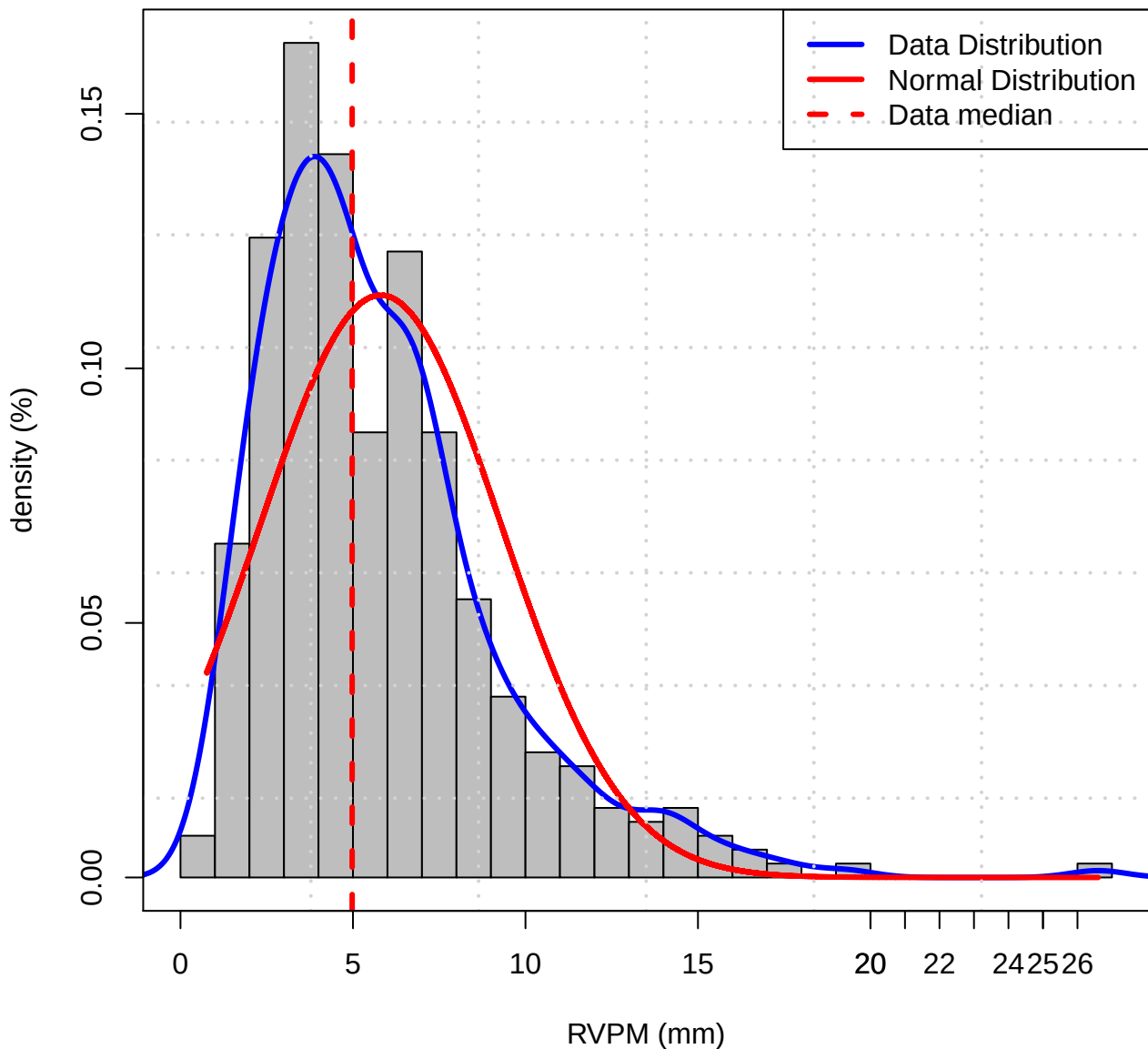
Histogram of Data distribution (PR of RVPM)
