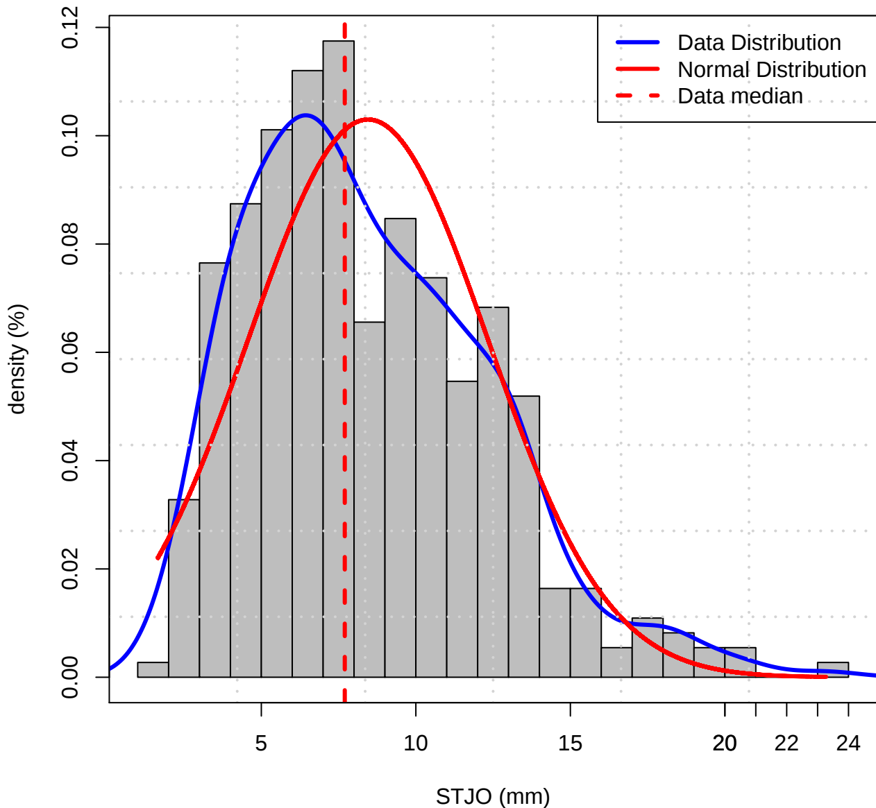
Histogram of Data distribution (PR of STJO)
