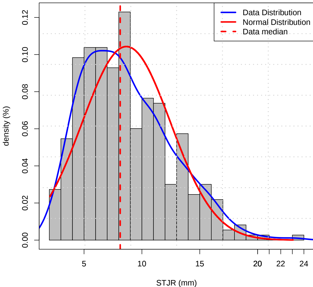
Histogram of Data distribution (PR of STJR)
