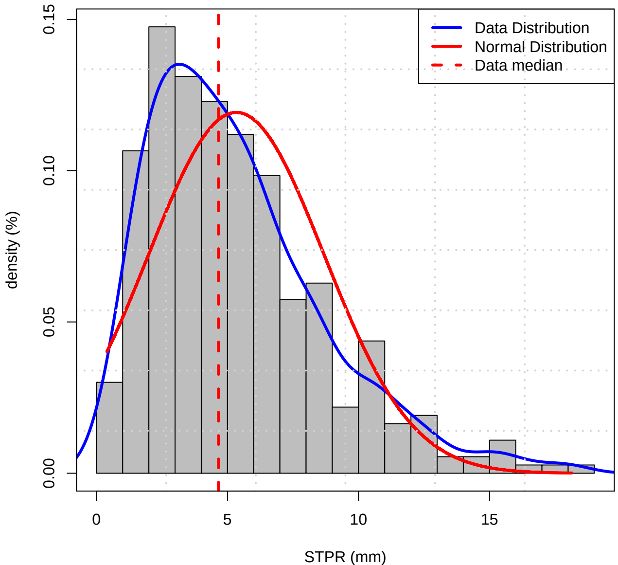
Histogram of Data distribution (PR of STPR)
