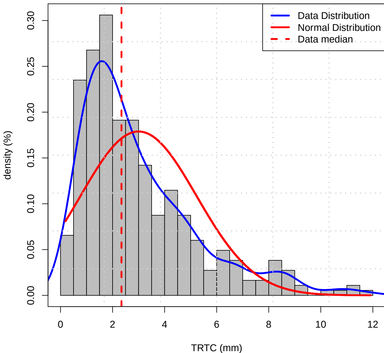
Histogram of Data distribution (PR of TRTC)
