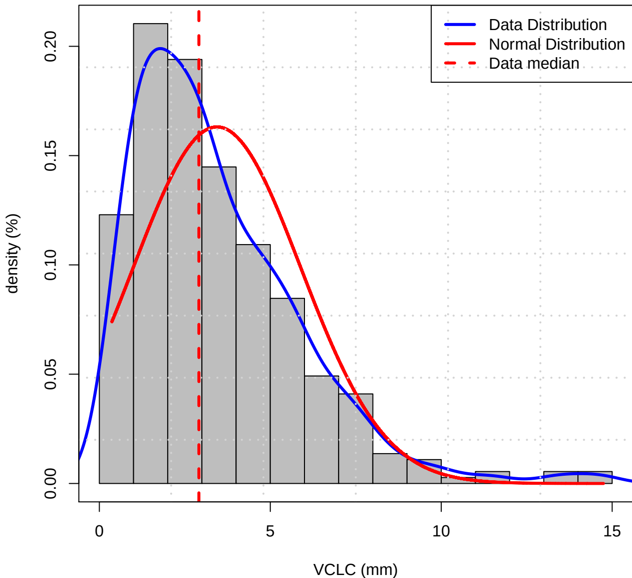
Histogram of Data distribution (PR of VCLC)
