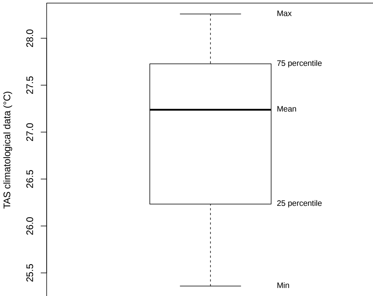
Box plot (TAS of STAN)
