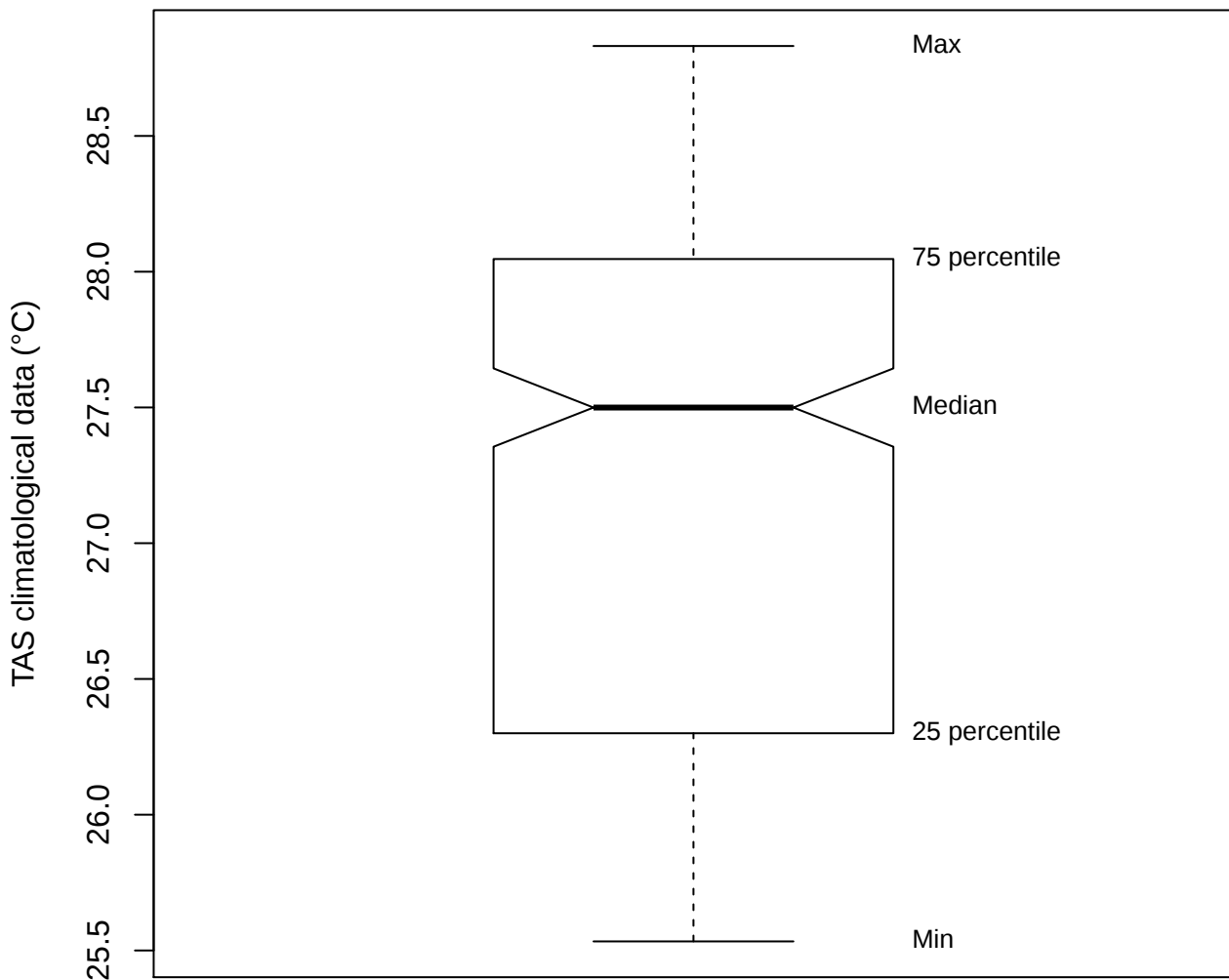
Box plot (TAS of TRTC)
