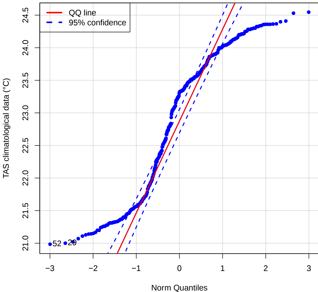
QQ plot (TAS of BLLF)
