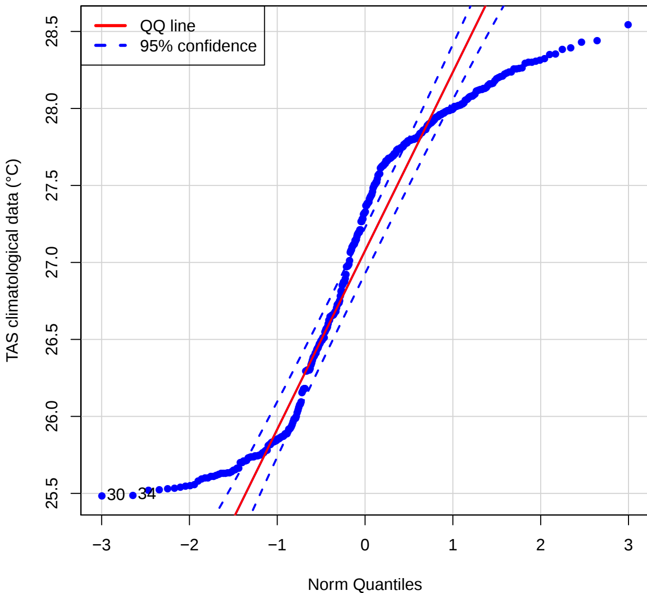
QQ plot (TAS of FDFL)
