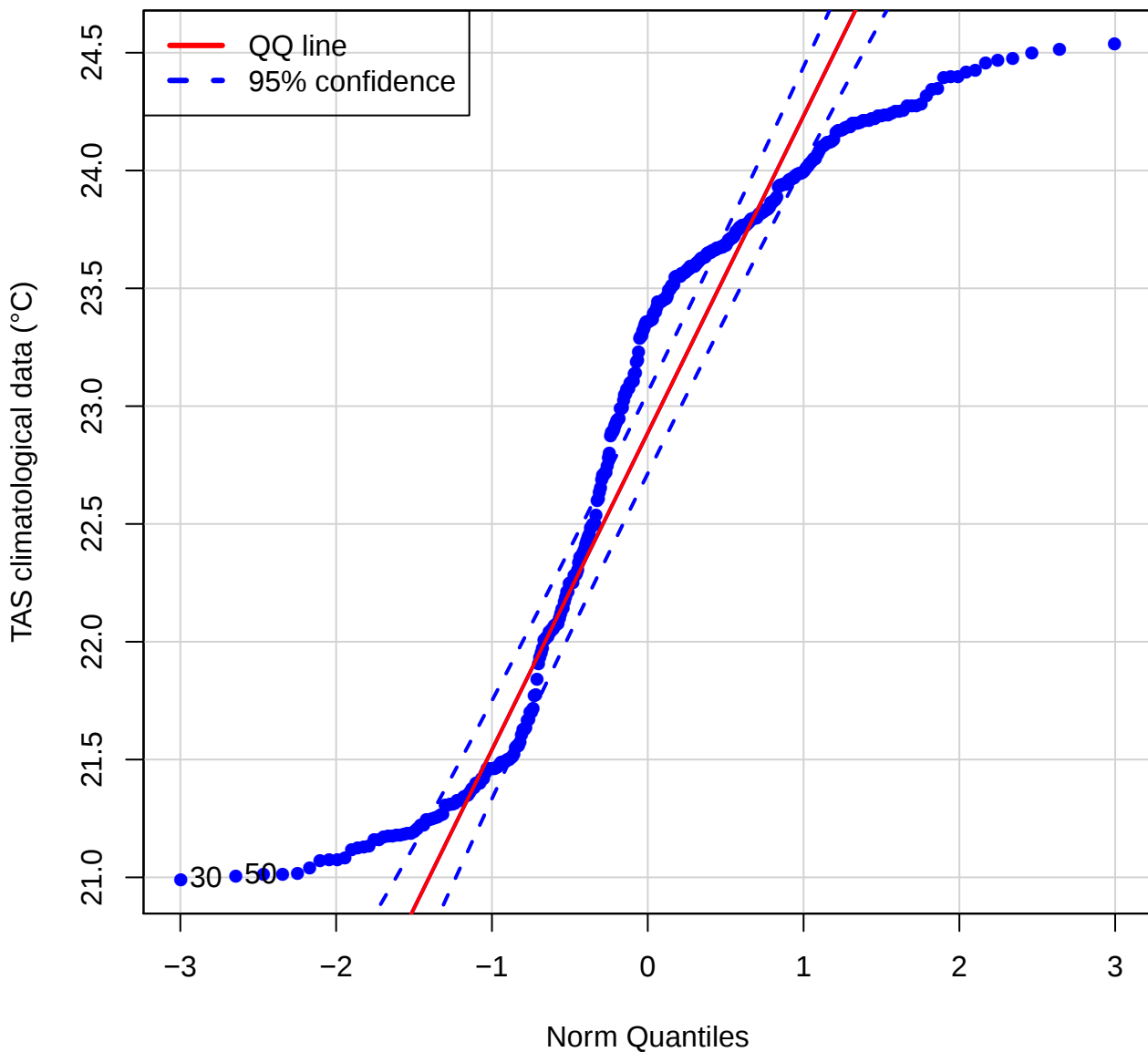
QQ plot (TAS of FSDC)
