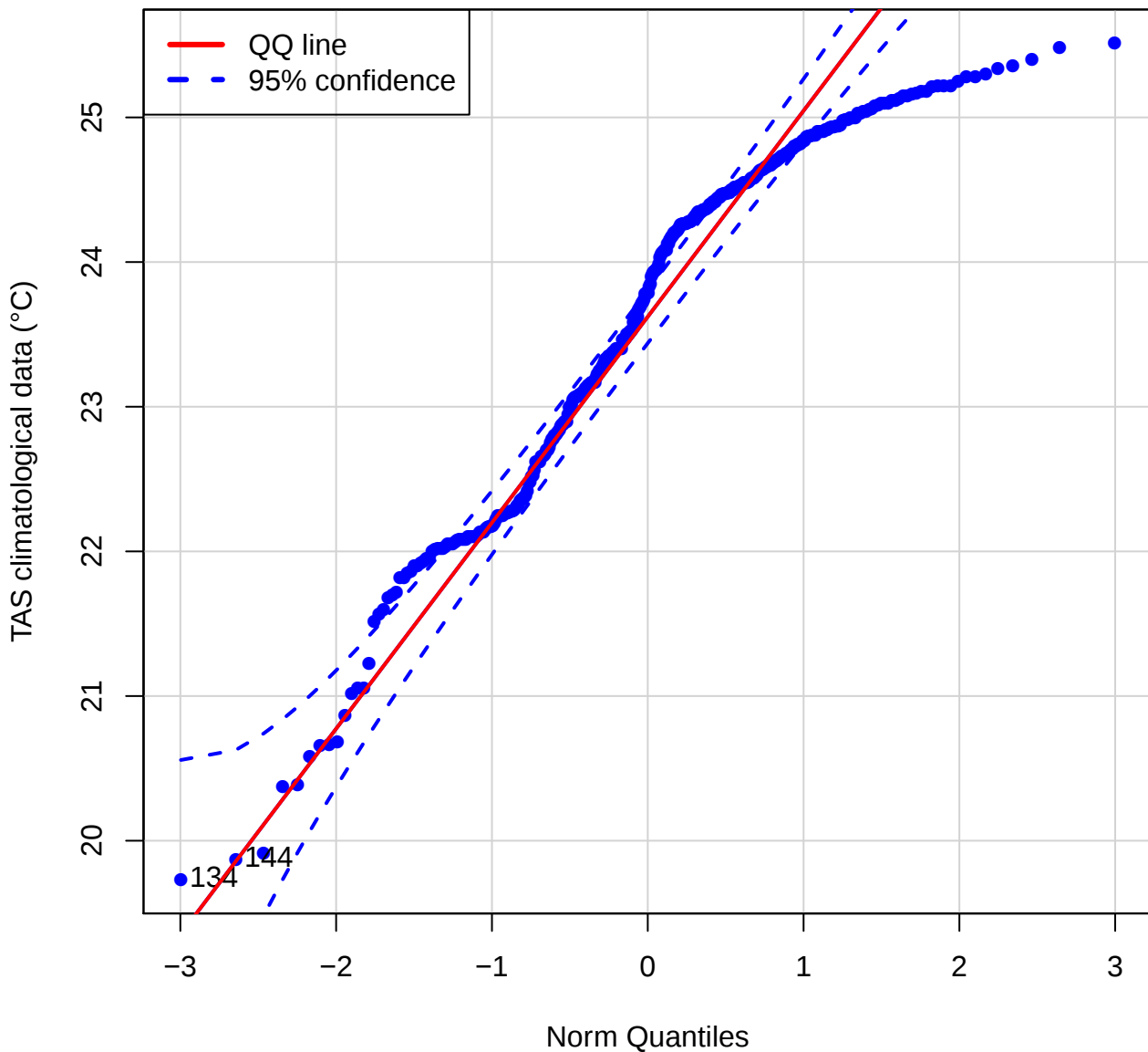
QQ plot (TAS of FSDG)
