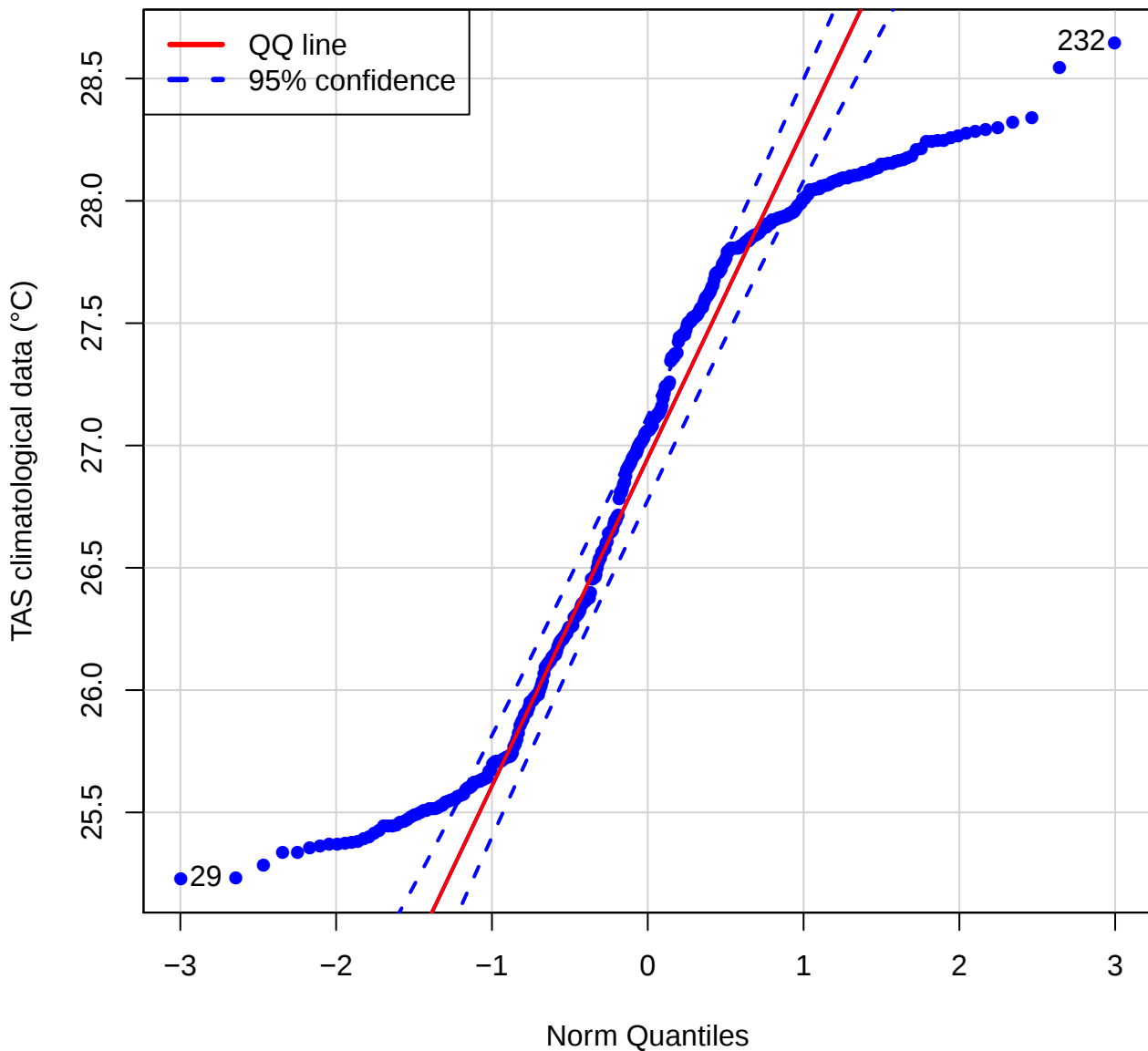
QQ plot (TAS of GDRV)
