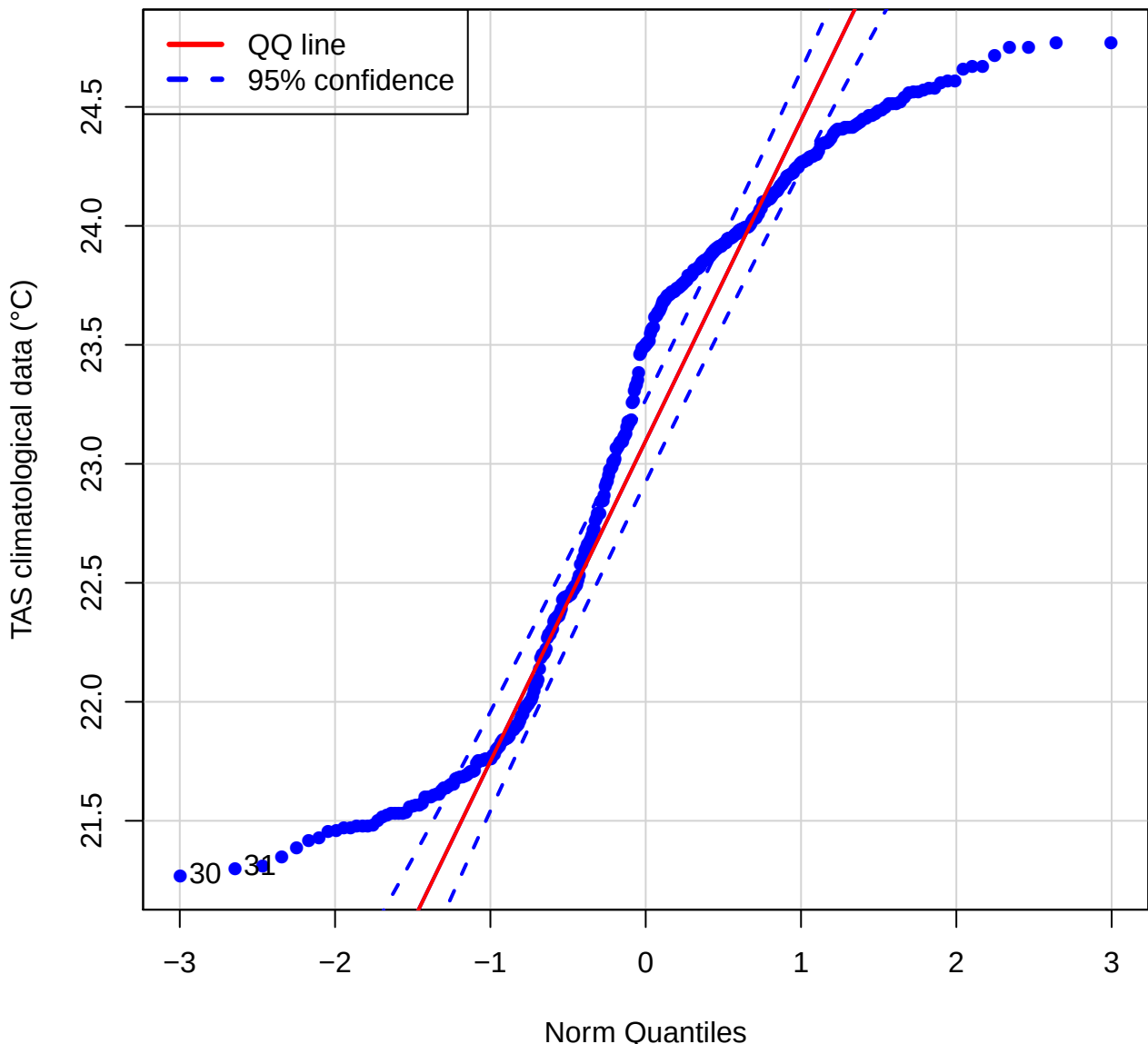
QQ plot (TAS of GMRN)
