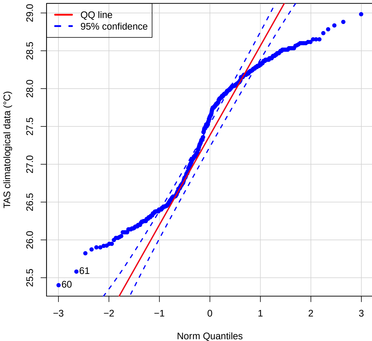
QQ plot (TAS of PANS)
