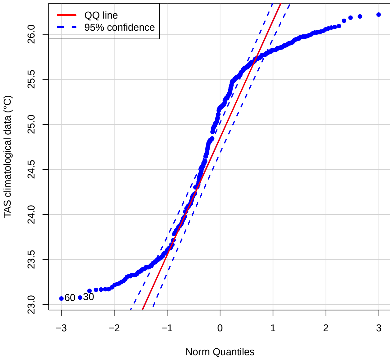
QQ plot (TAS of PECH)
