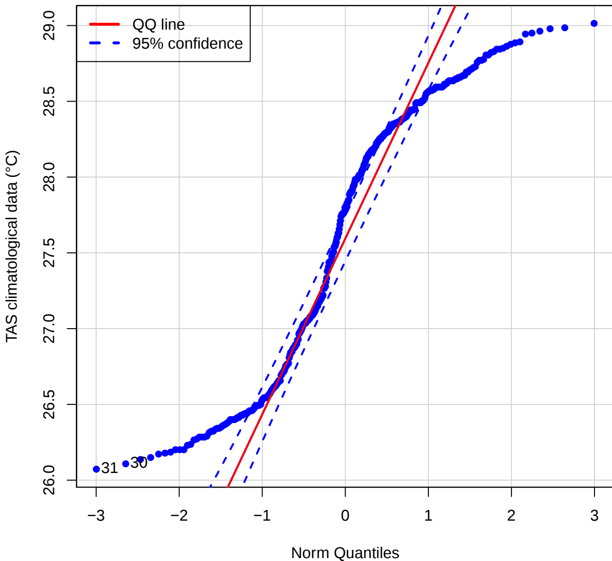
QQ plot (TAS of ROBP)
