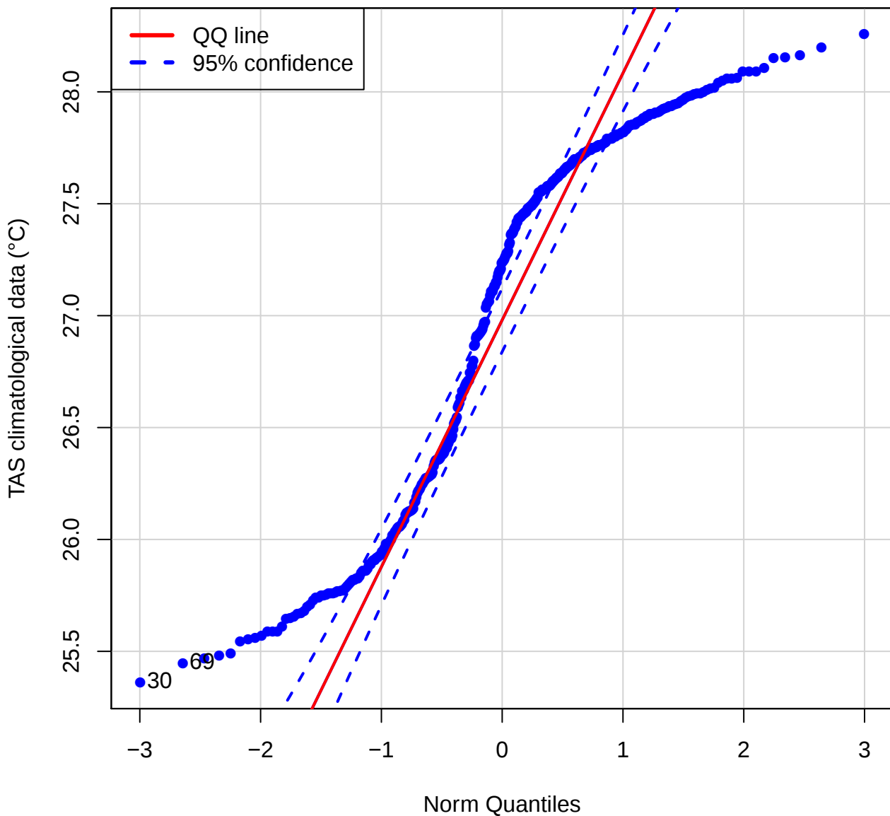
QQ plot (TAS of STAN)
