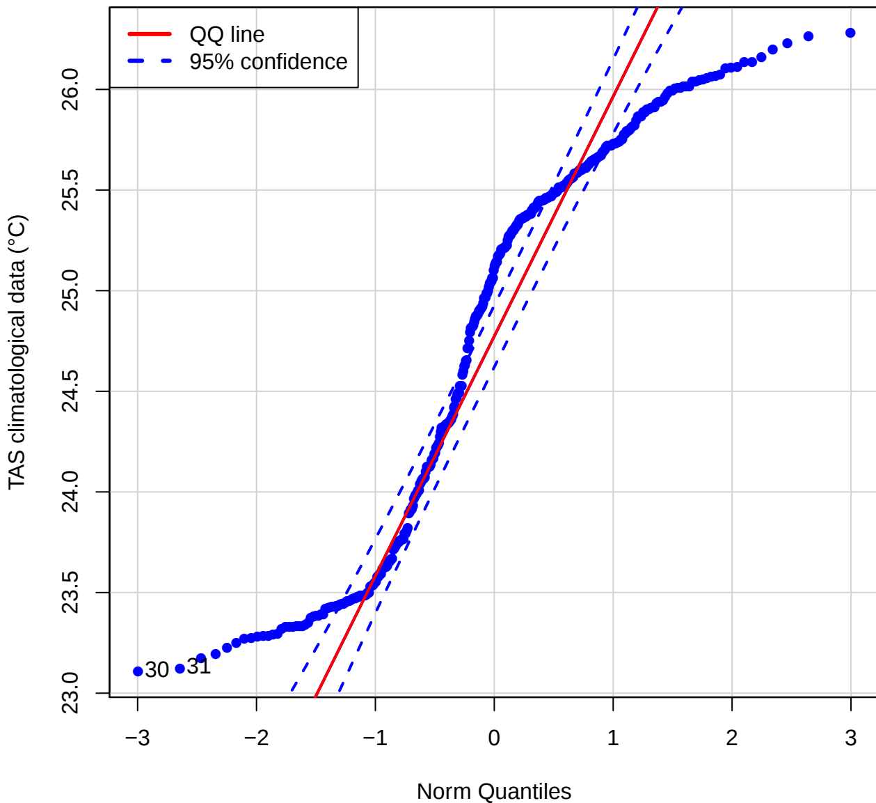
QQ plot (TAS of STEB)
