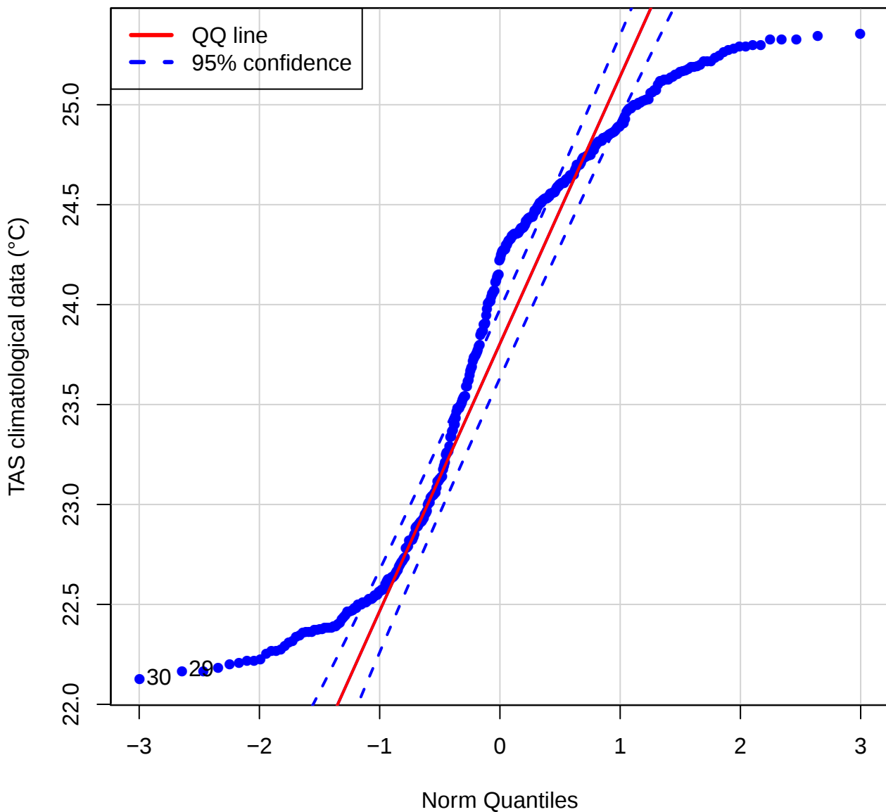
QQ plot (TAS of STJB)
