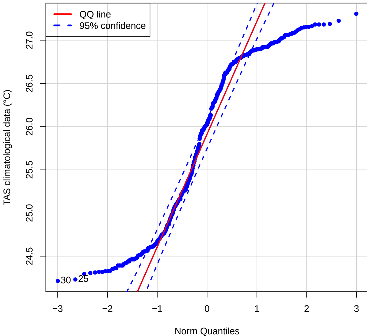
QQ plot (TAS of STJL)
