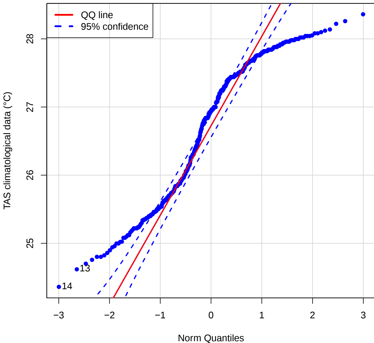
QQ plot (TAS of STLC)
