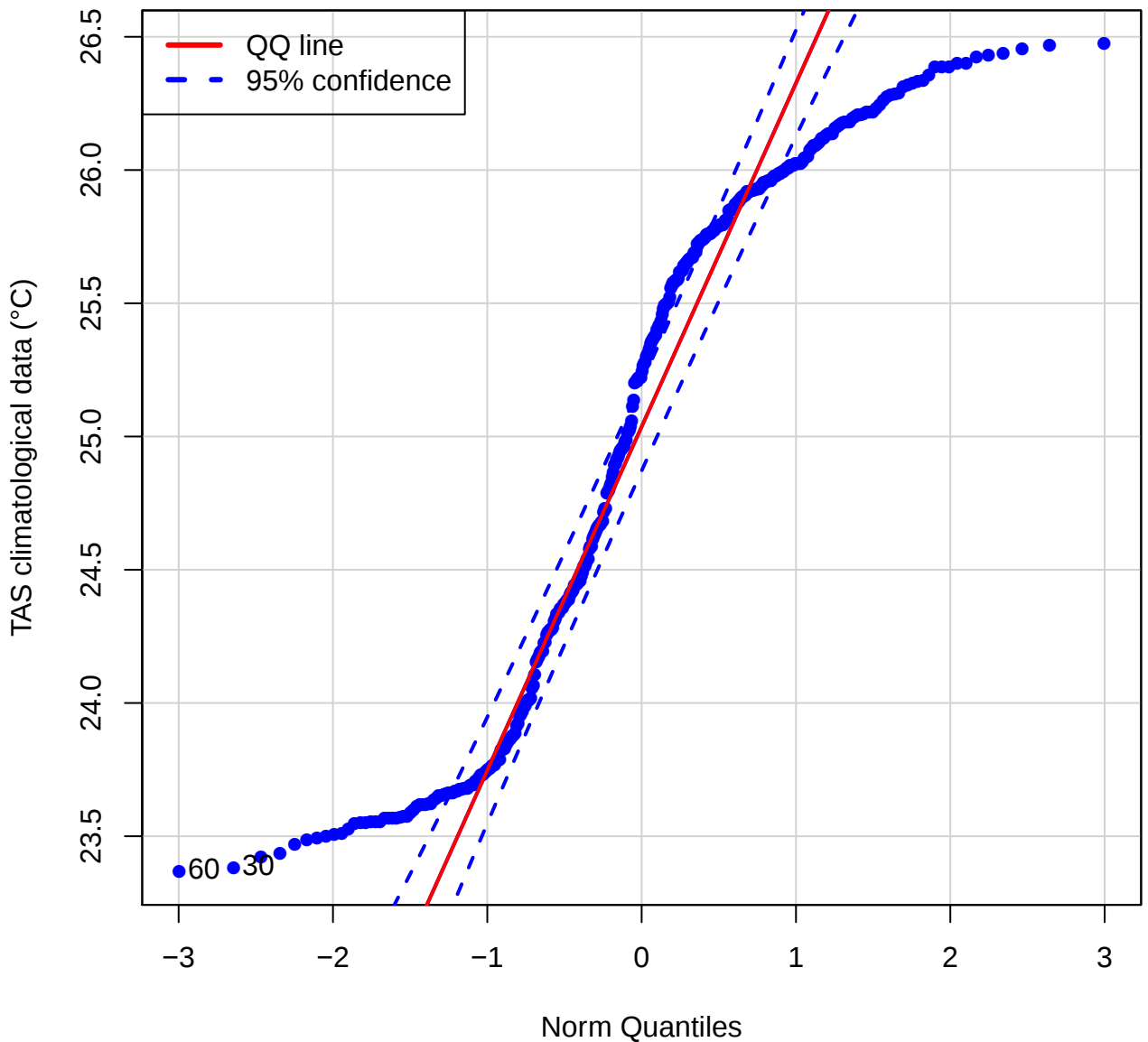
QQ plot (TAS of STMP)
