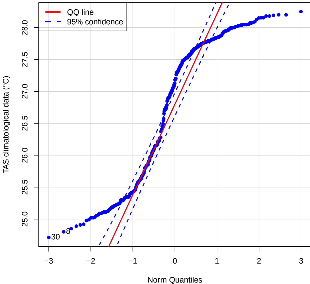
QQ plot (TAS of STPR)
