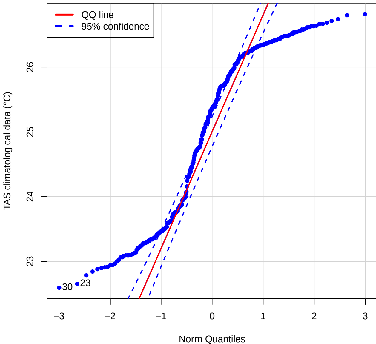
QQ plot (TAS of TILP)
