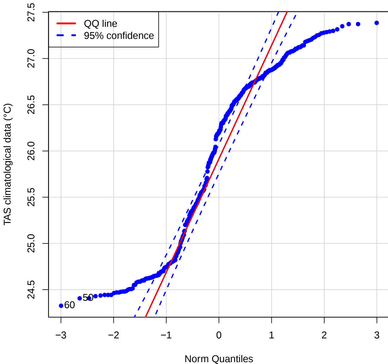
QQ plot (TAS of TRTR)
