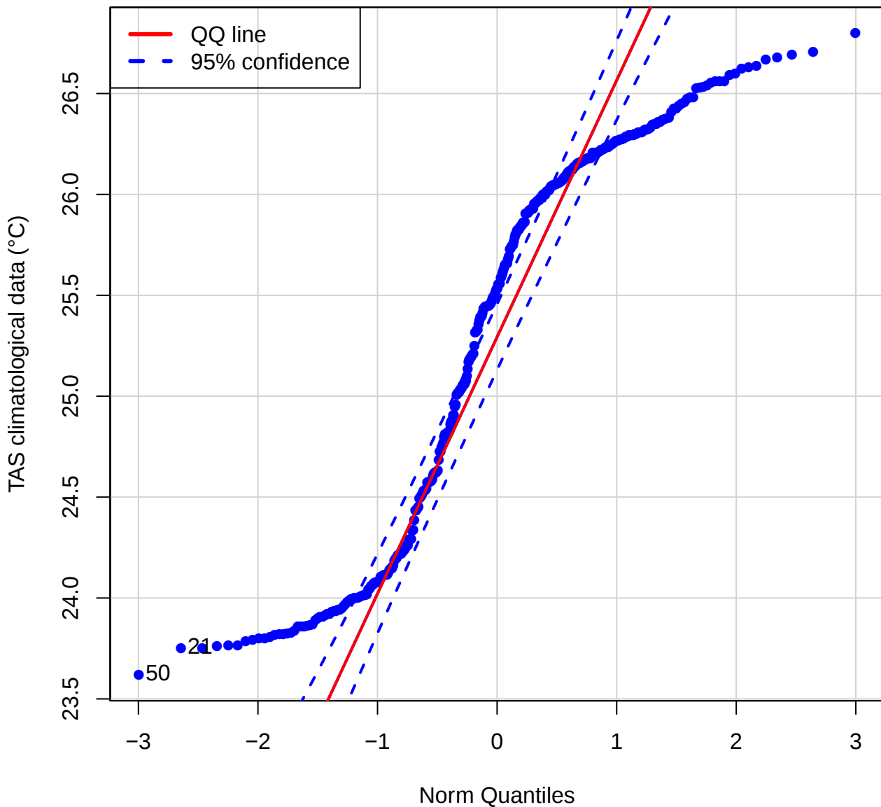
QQ plot (TAS of VCLR)
