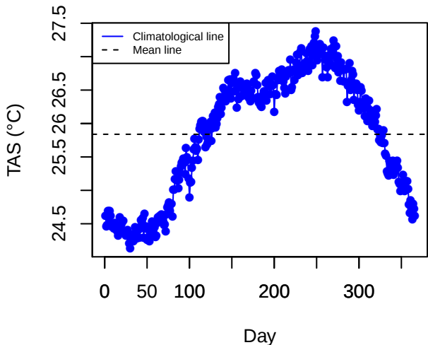
Climatology (FDFD)
