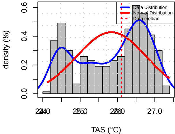
Histogram Distribution (FDFD)
