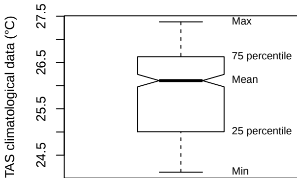
Box plot (FDFD)
