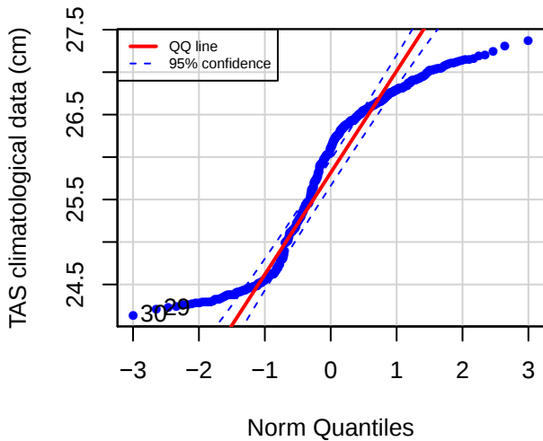
QQ plot (FDFD)
