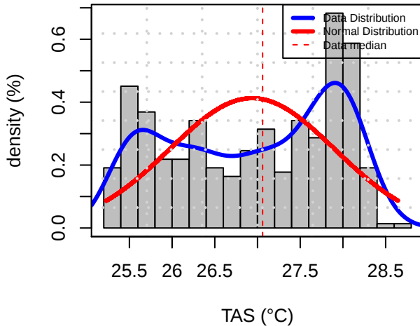
Histogram Distribution (GDRV)
