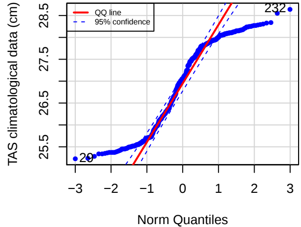
QQ plot (GDRV)
