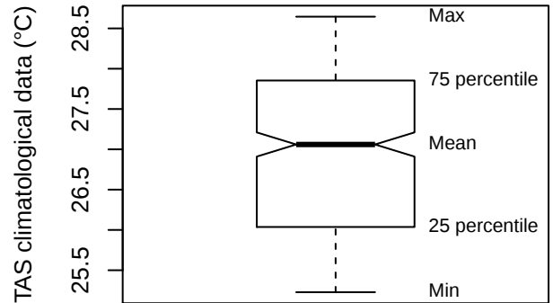
Box plot (GDRV)
