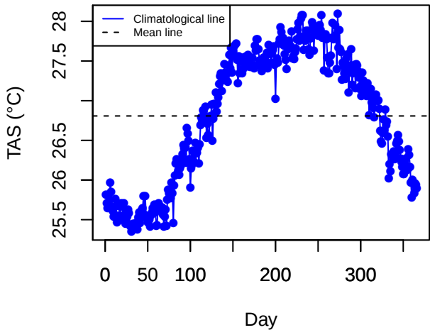
Climatology (LFRC)
