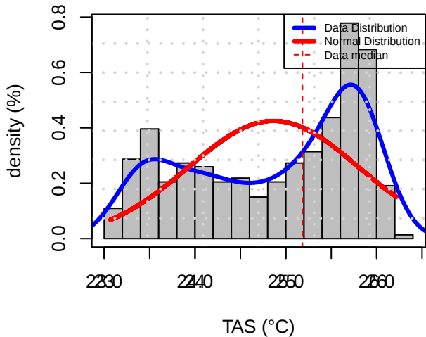
Histogram Distribution (PECH)
