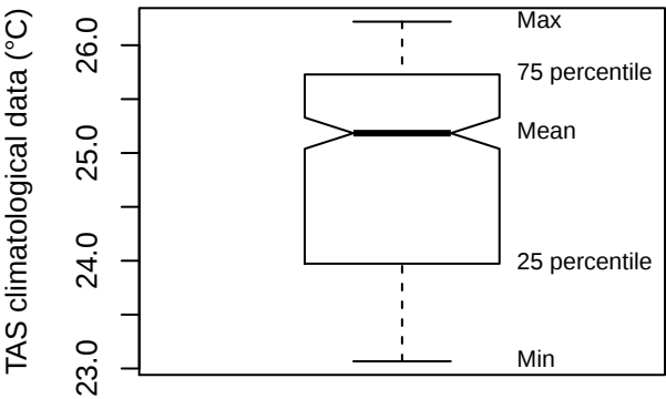
Box plot (PECH)
