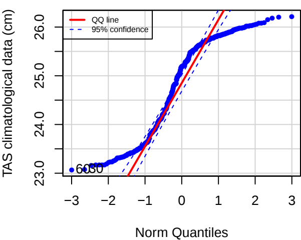
QQ plot (PECH)
