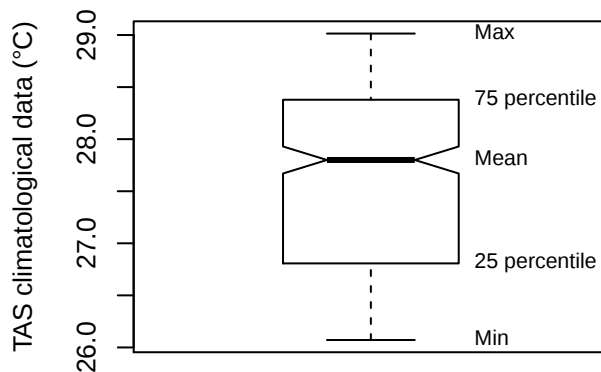
Box plot (ROBP)
