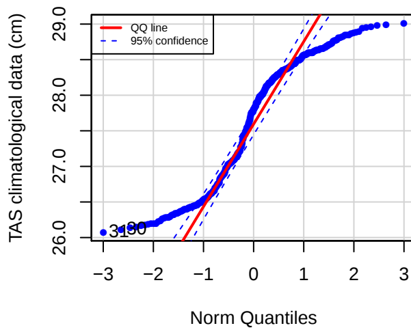
QQ plot (ROBP)
