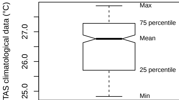
Box plot (RVPE)
