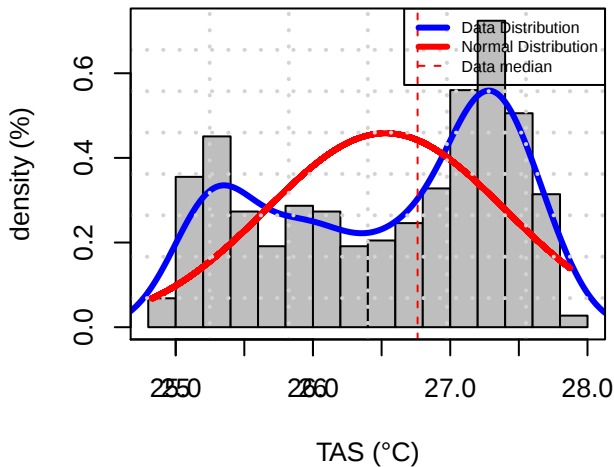
Histogram Distribution (RVPE)
