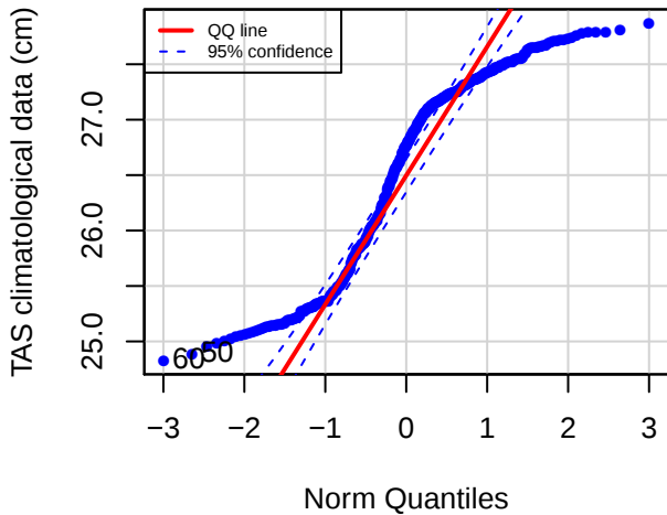
QQ plot (RVPE)
