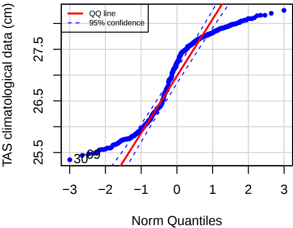
QQ plot (STAN)
