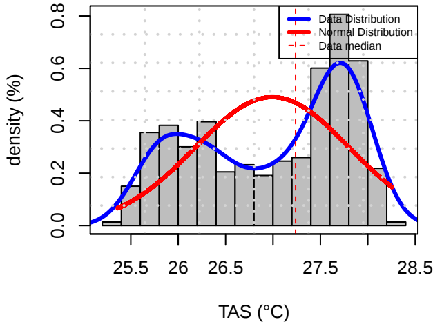
Histogram Distribution (STAN)
