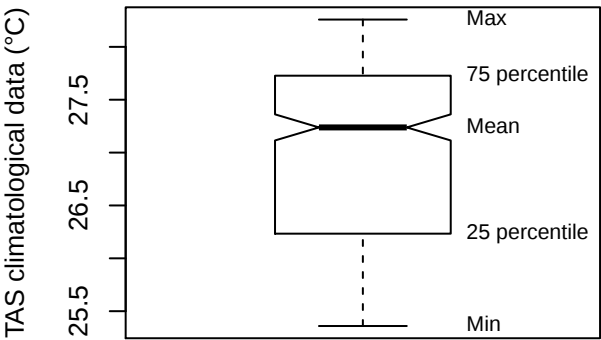
Box plot (STAN)
