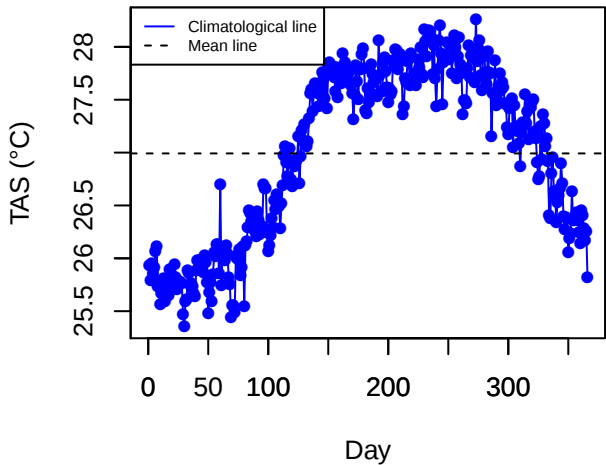
Climatology (STAN)
