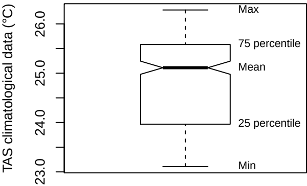
Box plot (STEB)
