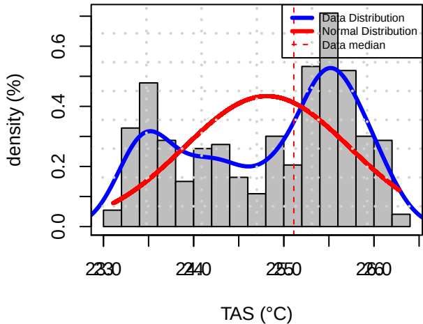
Histogram Distribution (STEB)
