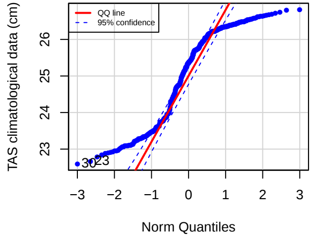
QQ plot (TILP)
