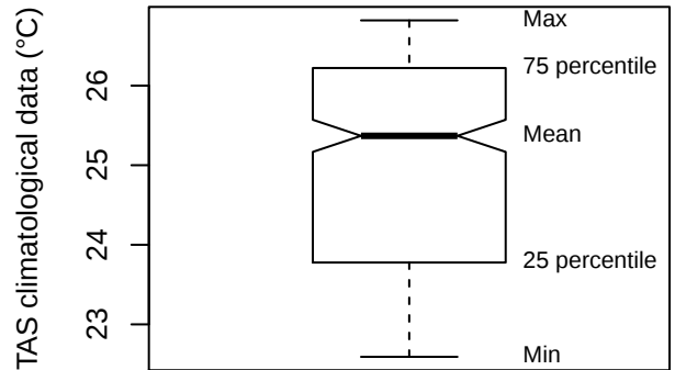
Box plot (TILP)
